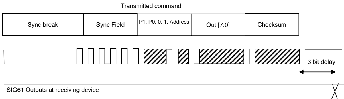
Figure 4.1 - Write command
